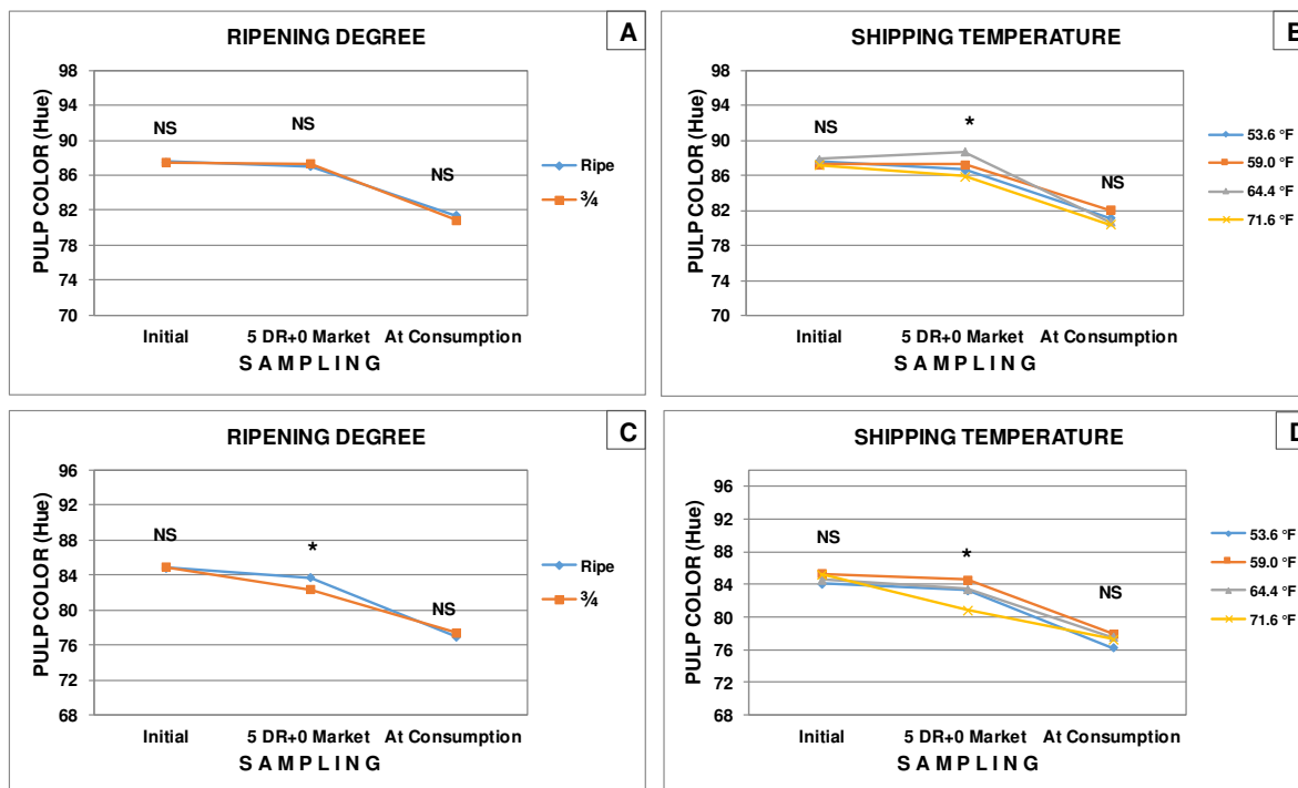
Figure 14. Effect of ripening degree (A, C) and shipping temperature (B, D) on pulp color (Hue) in Kent fruit with or without QHWT. RRTEM 2016.
