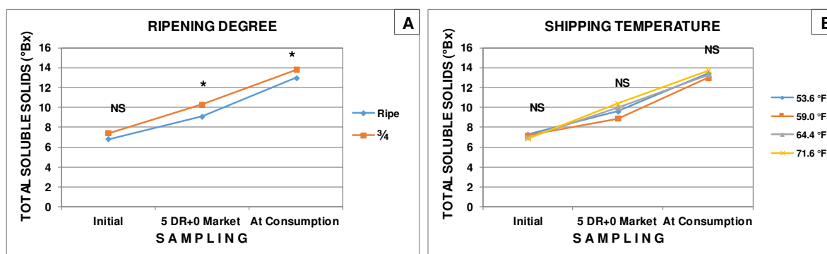
Figure 10. Effect of ripening degree (A) and shipping temperature on TSS content (°Bx) in Tommy Atkins fruit. RRTEM 2016.
