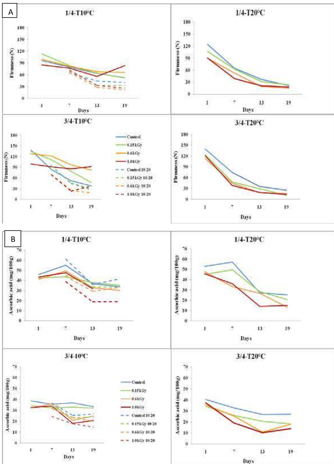
Figure 40 Changes in firmness (A) and ascorbic acid (B) in mango fruits cv 'Keitt' at different maturity stages ( \frac{1}{4} and \frac{3}{4} ), irradiated at different doses and stored at 10 and 20°C. Dotted lines indicate the transfer of fruits from 10 to 20
